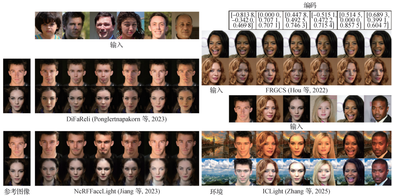
图5 DiFaReli、NeRFFaceLight、FRGCS和ICLight算法在对应光照条件(参考图像、光照编码和环境地图)下的结果 Fig. 5 The results of the DiFaReli, NeRFFaceLight, FRGCS and ICLight algorithms under corresponding lighting conditions (reference images, light codes and environment maps)
